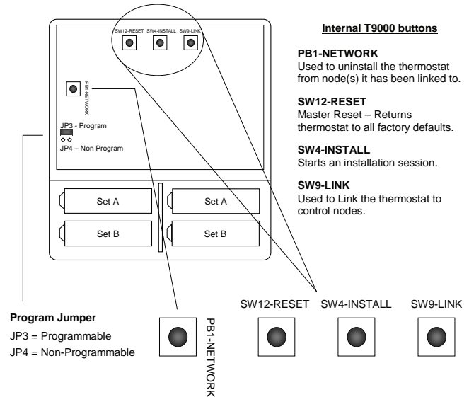
Figure 8. Internal Buttons
