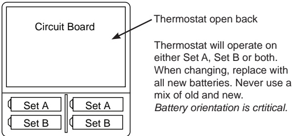
Figure 3. Battery Location
