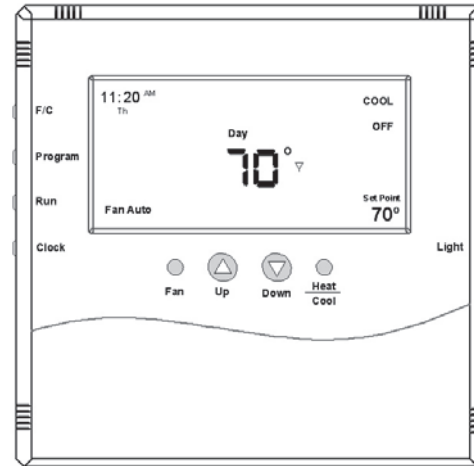
Figure 1. T9000 Front View
