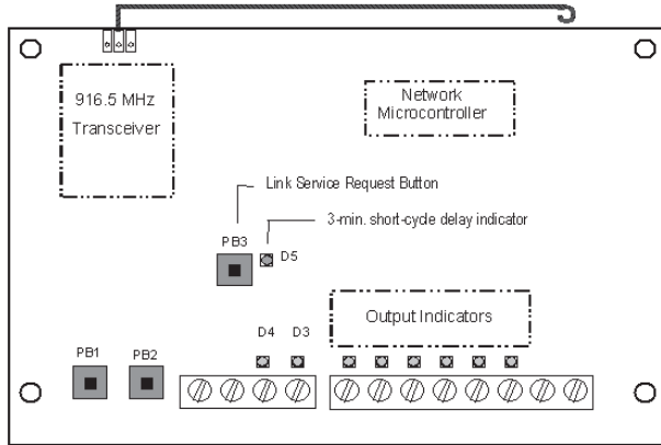
Figure 10. PTAC Wireless Control Node
